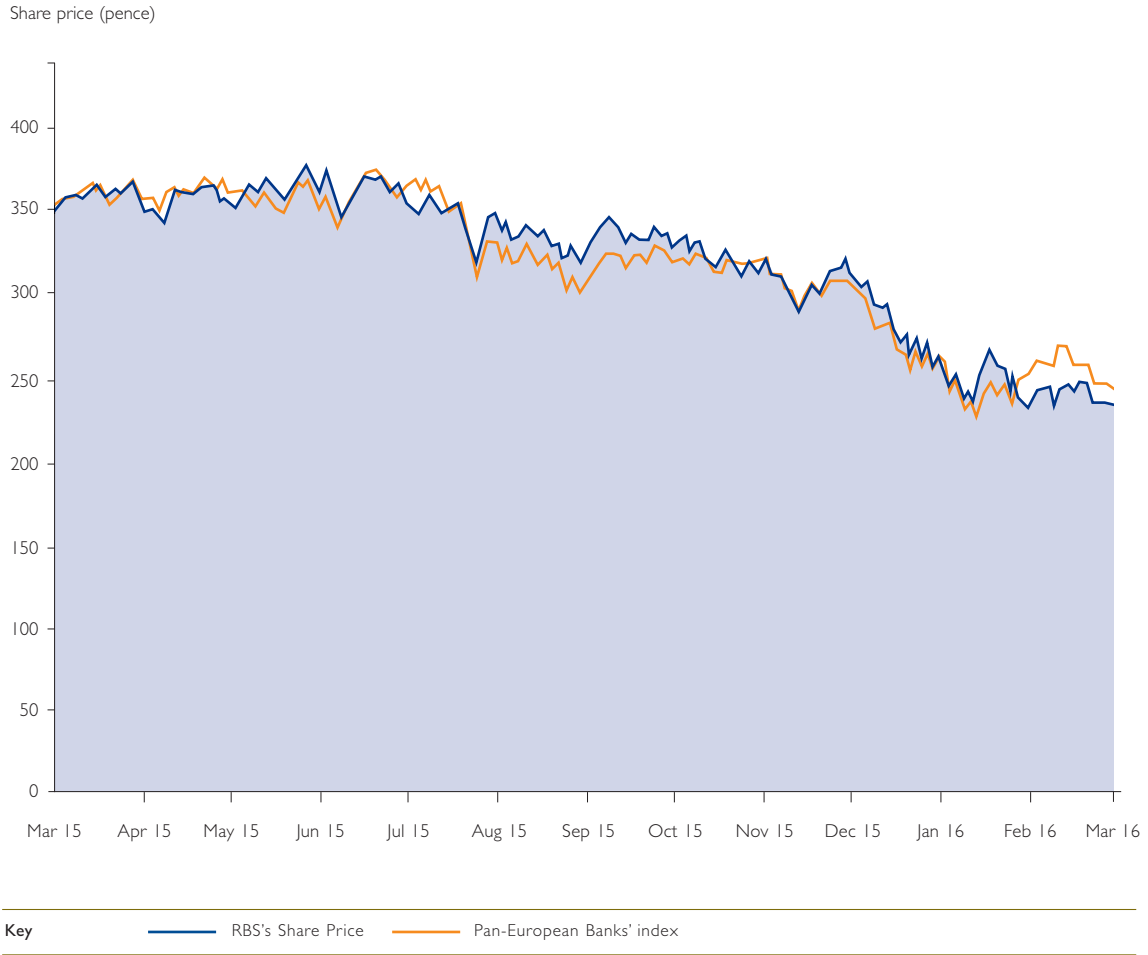
Figure 2.1: RBS's share price performance
