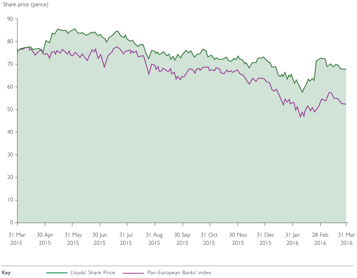
Figure 3.1: Lloyds share price performance
